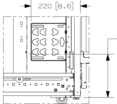
PDU BRACKET DETAIL
