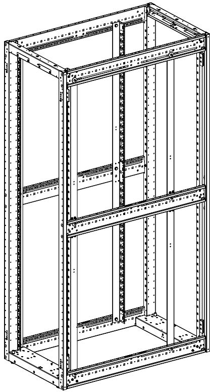
600mm E-RAIL ARRANGEMENT NO PASS THRU OPENINGS
