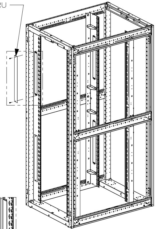
800mm E-RAIL ARRANGEMENT
