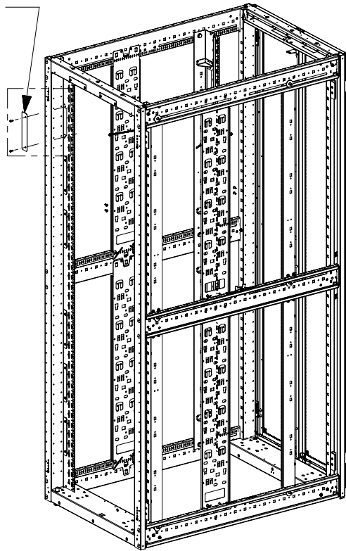
700mm E-RAIL ARRANGEMENT
